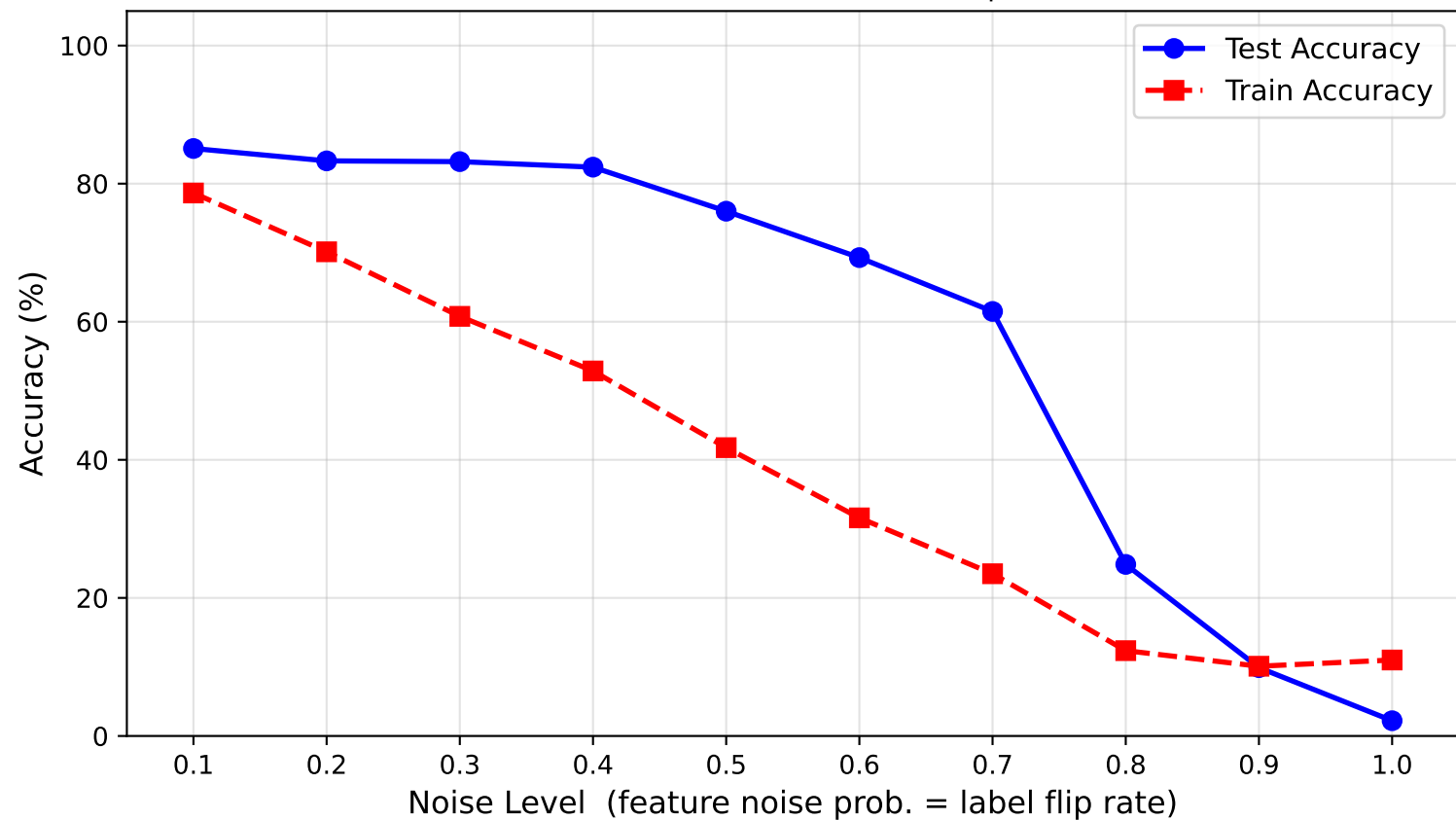
MNIST Accuracy vs. Noise Level (Vacuous trust · 16 neurons · 20 epochs)
